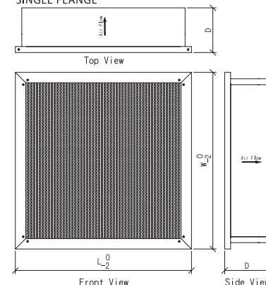
*SINGLE FLANGE
